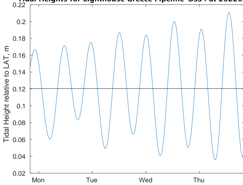
Tidal Heights for Lighthouse Greece Pipeline-OSS4 at 20220424
